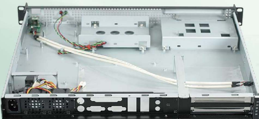
Internal Structure and Rear Side Panel
